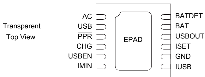
Figure 3. 34676 Pin Connections
