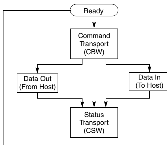
Figure 3-4. Bulk-Only Transport Flowchart
